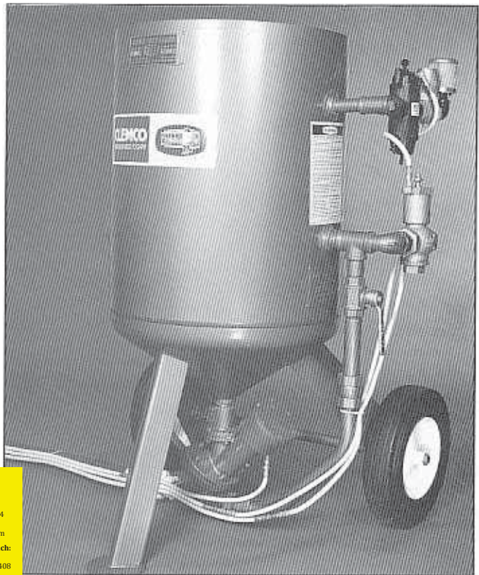
Sentinel Pneumatic Remote Control System with TLR-300
